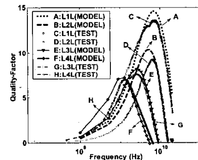
Fig. 6. Comparison Q: test value and model value (Same inductors as in Figure 5, but on LRS)
