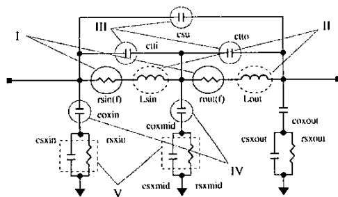
Fig. 4. A universal inductor model
