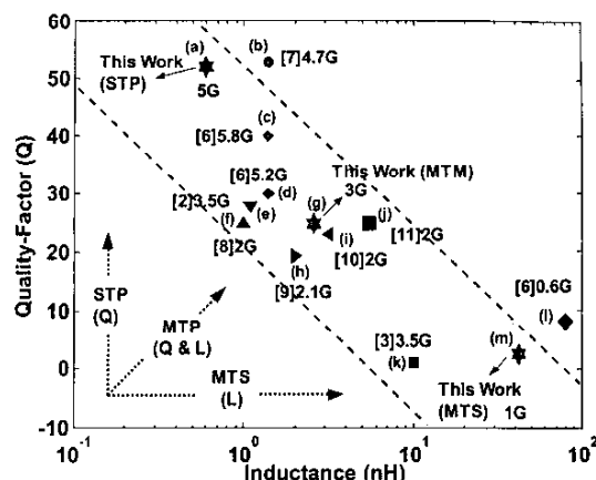
Fig. 10. Inductance versus Q (The numbers near the symbols are the reference number and the frequency in GHz.)
